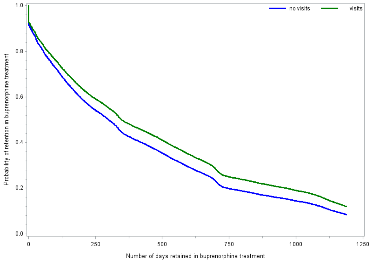
Figure 2: Kaplan Meir Survival analysis on probability of retention in buprenorphine treatment among patients with opioid use disorder initiated on buprenorphine in 2011: Impact of receipt of outpatient psychotherapy
