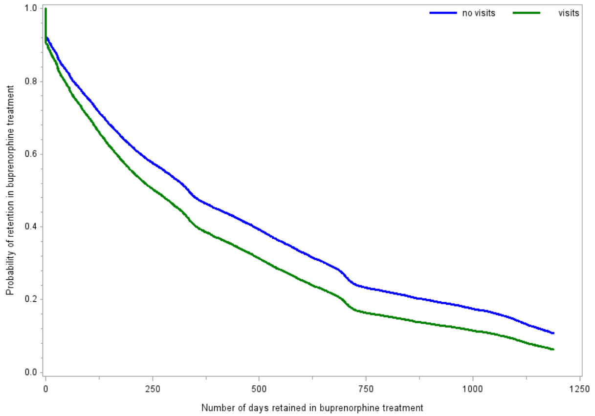
Figure 1: Kaplan Meir Survival analysis on probability of retention in buprenorphine treatment among patients with opioid use disorder initiated on buprenorphine in 2011: Impact of inpatient hospital mental health admissions
