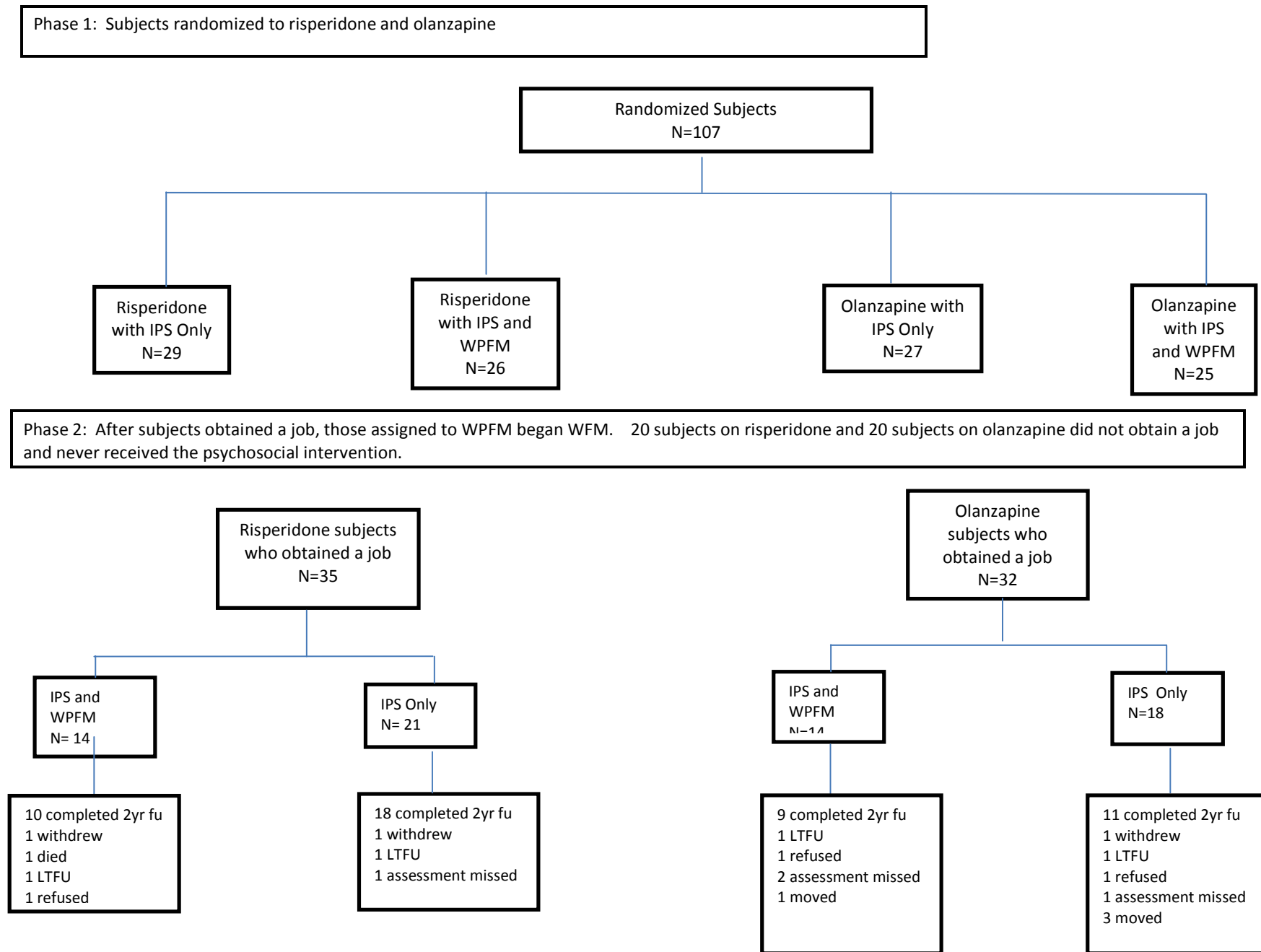
Figure 1 CONSORT CHART
